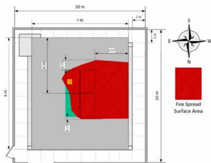
Total fire spread across PIR insulation roof assembly.
